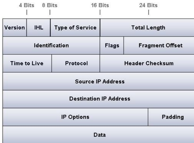
Fig. 1 Packet format of VoIP
