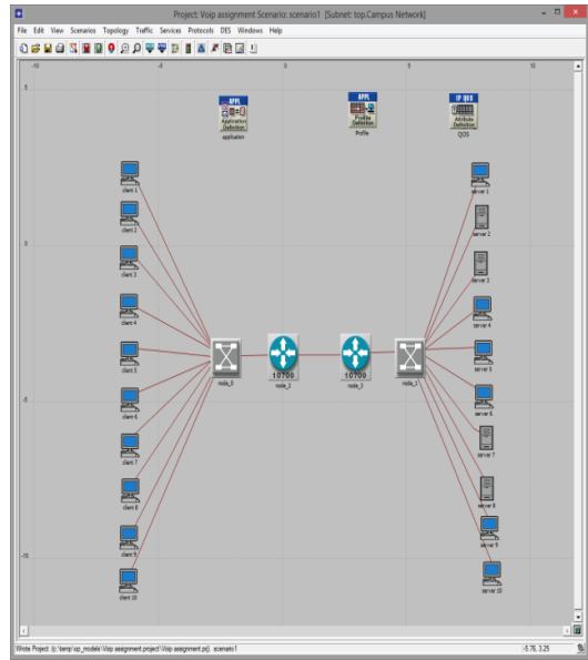
Fig. 4 IP topology
