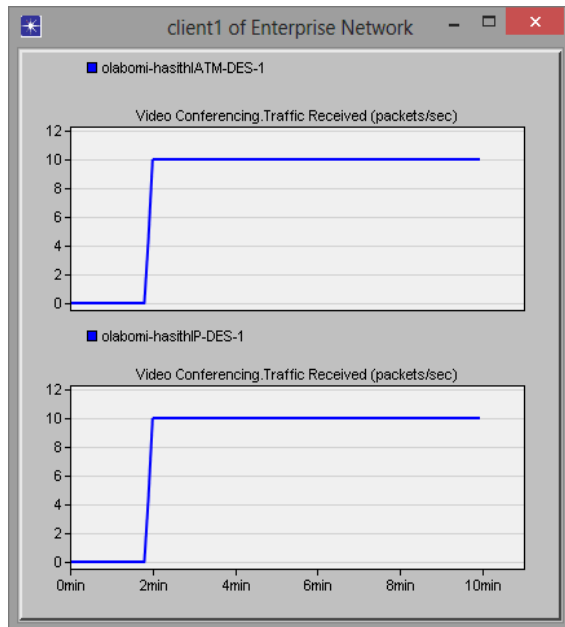
Fig. 5 Video Conference Traffic received in Packet/sec.
