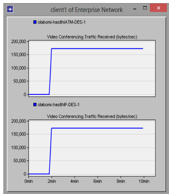
Fig. 6 Video conference Traffic received in bytes/sec
