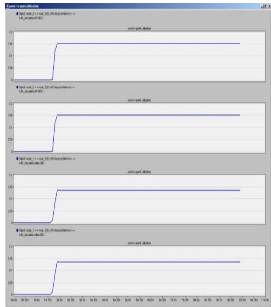
Fig. 10 Point-To-Point Utilization
