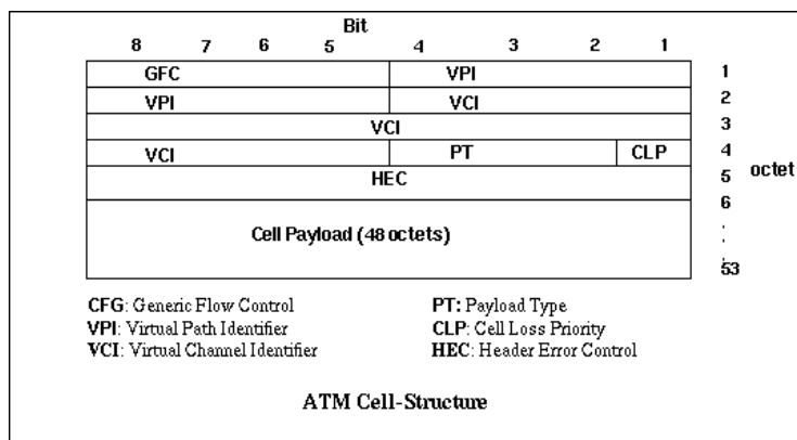
Fig. 2 ATM cell structure.
