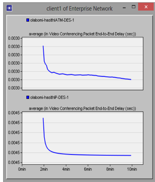
Fig. 8 End-to-end packet delay
